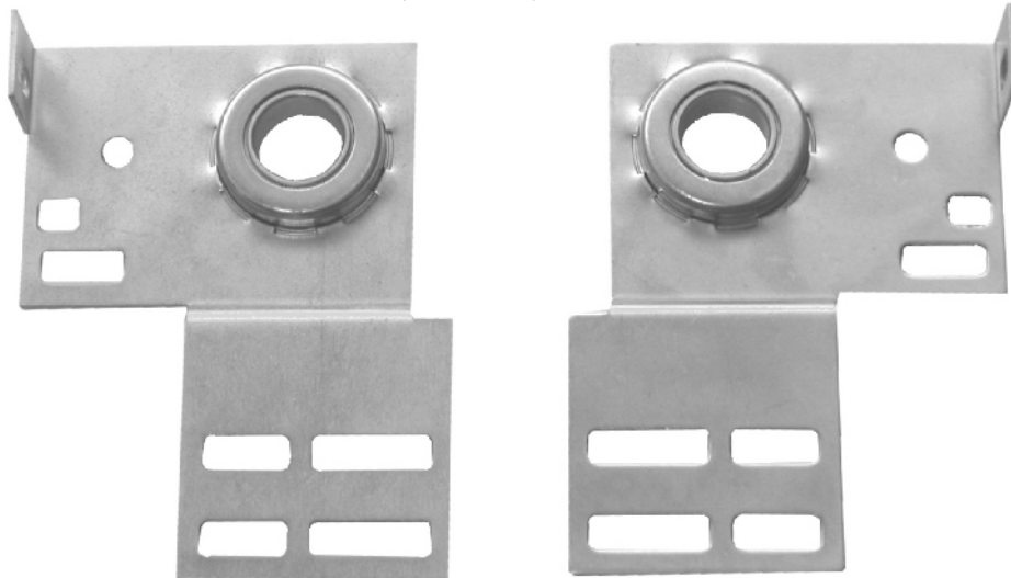
Offset End Bearing Fixture, 3-3/8"
